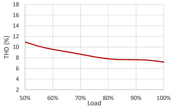
THD vs Load (230V/50Hz)
