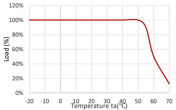
Load vs temperature ta
