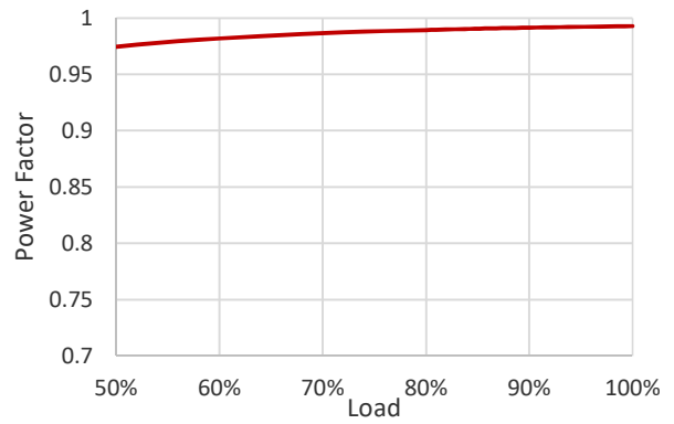
Power Factor vs Load (230V/50Hz)
